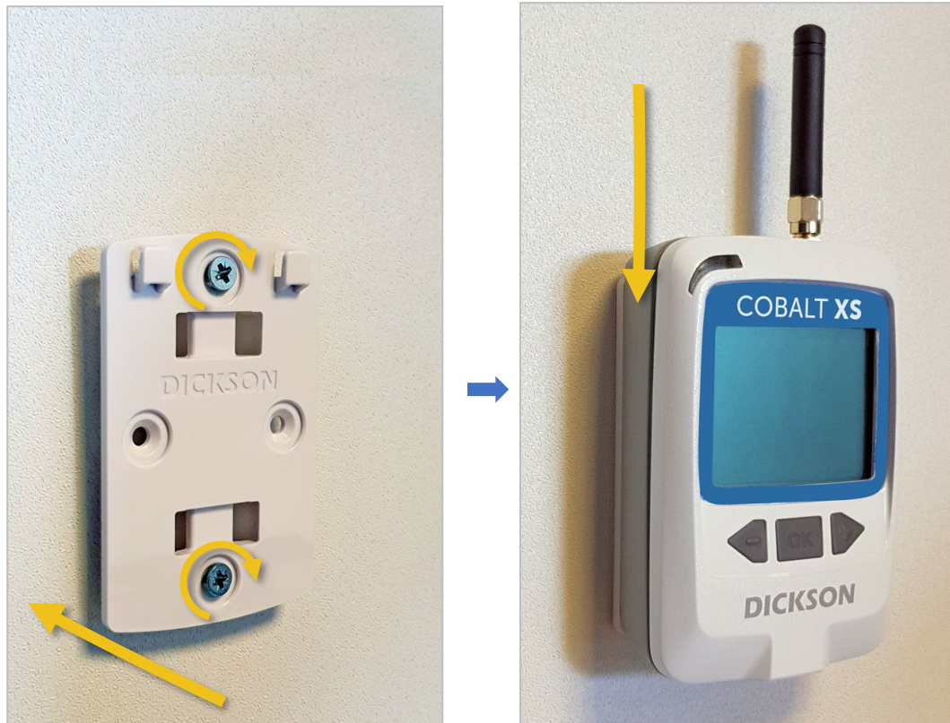
Figure 12 – Mounting the Cobalt XS with the wall-mount plate
