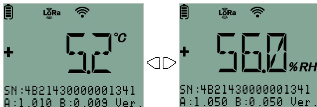
Figure 16 – Sensor information for a dual temperature and relative humidity sensor
